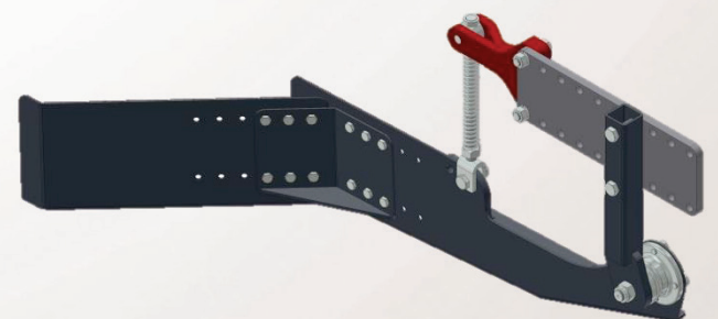
Paraterra flottante Floating soil deflector
