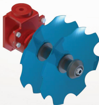
Dischi-folli Mini harrow plow discs (to cover the plant)
